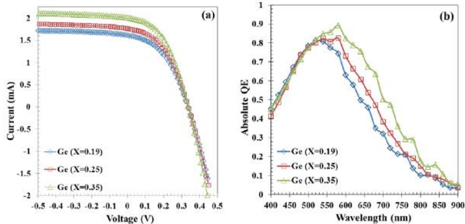
Figure 7. (a) IV curves and (b) Absolute QE vs. Wavelength for nc-SiGe:H solar cells with varying Ge content with optimum PH 3 flow (i-layer Thickness ~ 0.7 \mu m)
