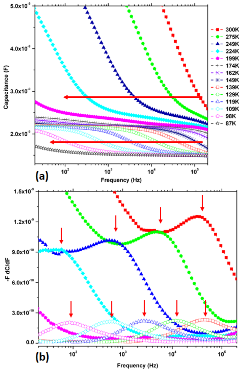
Figure 4.28 (a) CFT data for nc-SiGe:H solar cell ( X_{Ge}=0.35 ). The red arrows indicate the capacitance shift due to two different trap levels. (b) Differential capacitance curves. Arrows indicate emission peaks.
