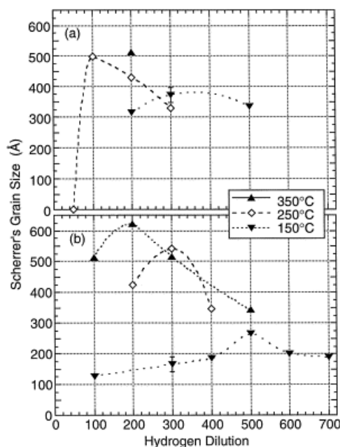
Figure 2.19 Grain sizes versus hydrogen dilution for nc-SiGe:H samples deposited at (a) 0.5mT, 89mW/cm 2 and (b) 0.9mT, 637mW/cm 2 at different temperatures [76]
