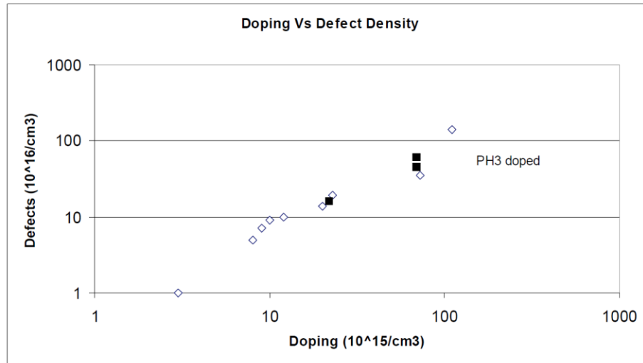
Figure 2.14 Effect of PH3 doping on defects in nc-Si:H solar cell [66]
