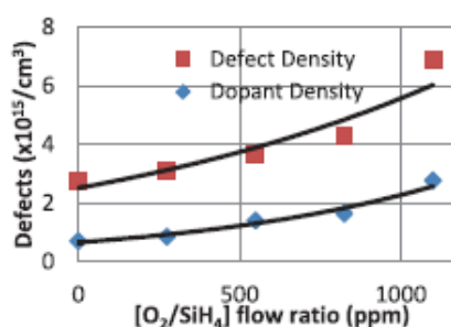
FIG. 4. Dopant and defect density values obtained from capacitance-voltage measurements versus oxygen flow during growth.
