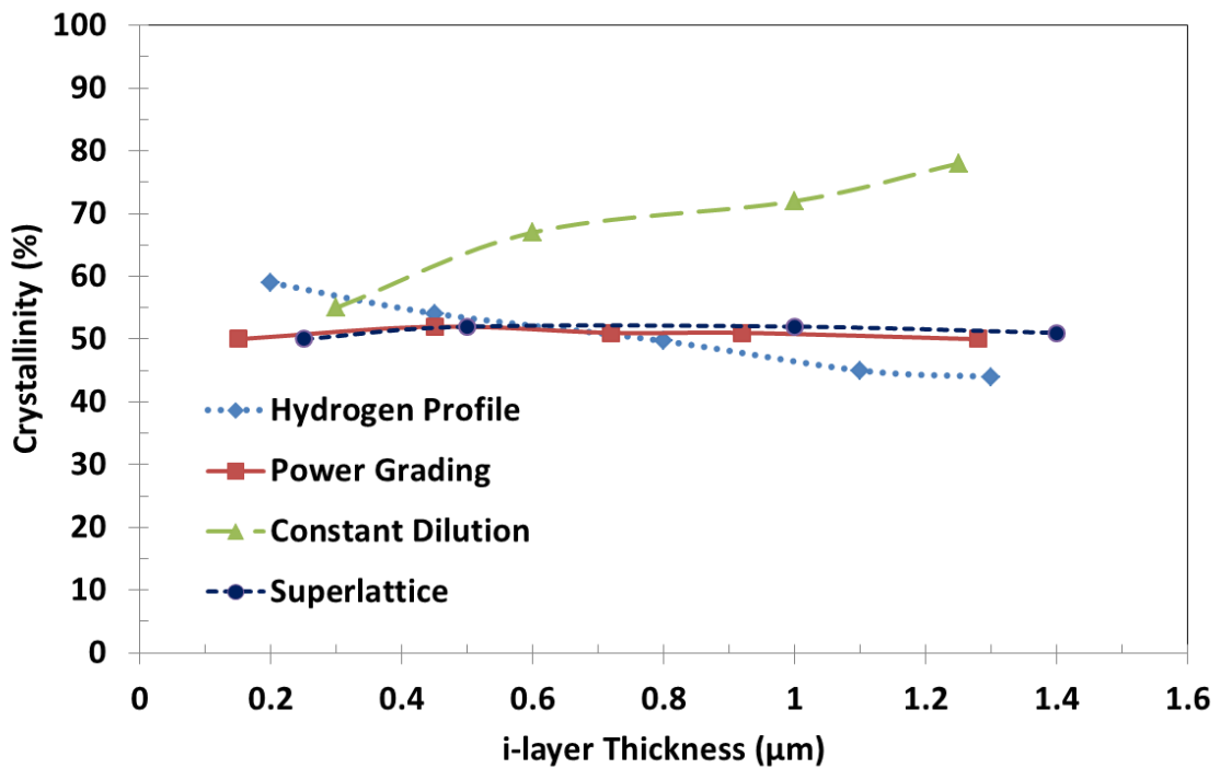
Figure 4.7 Crystallinity vs. i-layer thickness in nc-SiGe:H film
