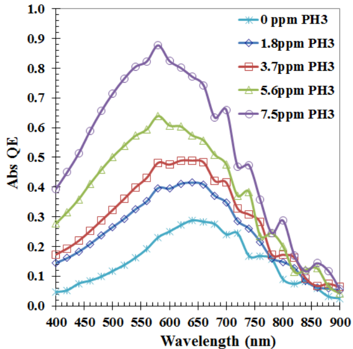
Figure 4.20 Absolute QE vs. Wavelength for nc-SiGe:H solar cells with ( X_{Ge} \sim 0.35 ) for varying PH_3 flow rates
