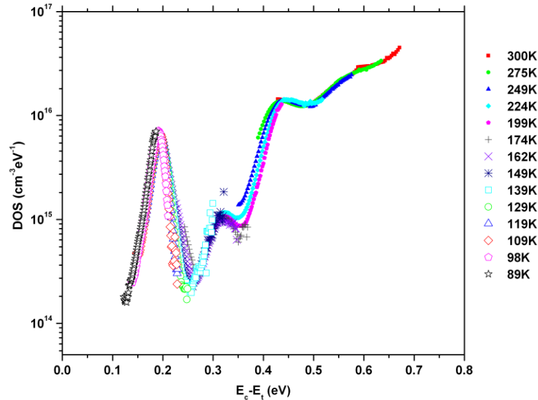
Figure 4.30 Calculated defect density profile of nc-SiGe:H solar cell ( X_{Ge}=0.35 )
