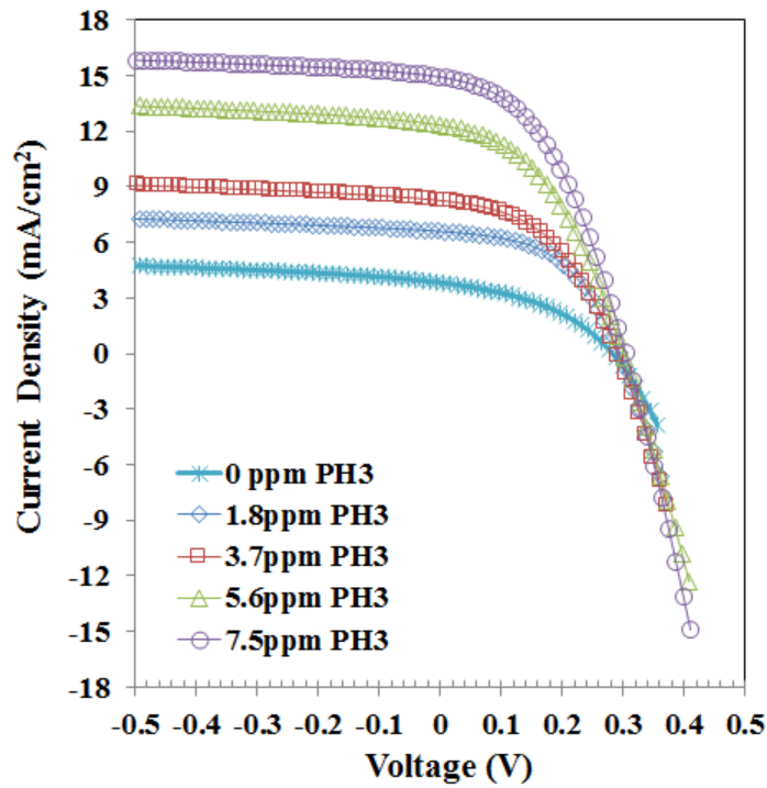
Figure 4.19 JV curves and for nc-SiGe:H solar cells with ( X_{Ge} \sim 0.35 ) for varying PH_3 flow rates
