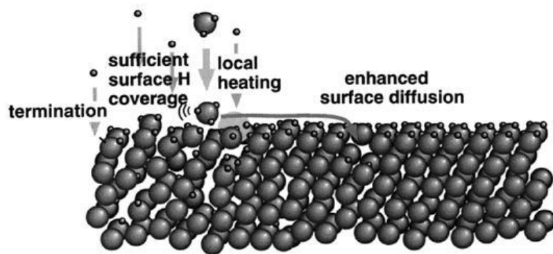
Figure 2.3 Surface diffusion model for the growth of ncSi:H material [54]
