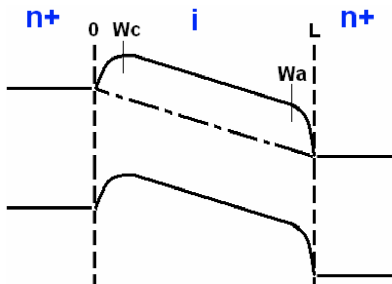
Figure 3.12 Band diagram of an n-i-n device under electrical bias [104]
