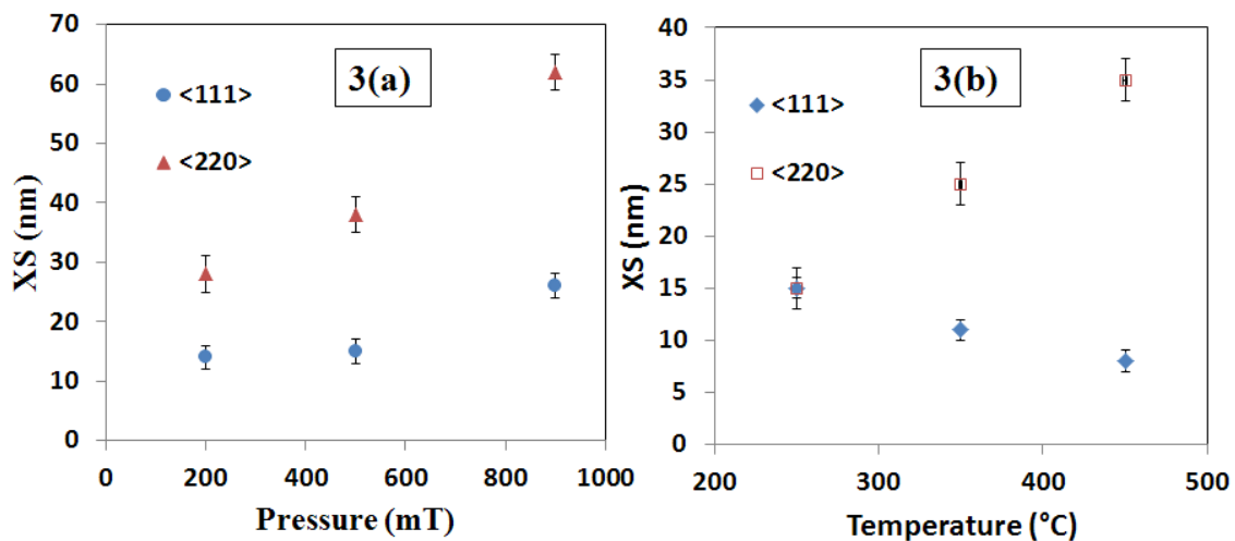
Figure 3. (a) Grain size of nanocrystalline Ge:H films grown at 300C, (b) Grain size of nanocrystalline (Si,Ge):H films grown at 900 mT (Si:Ge ~ 1:1)
