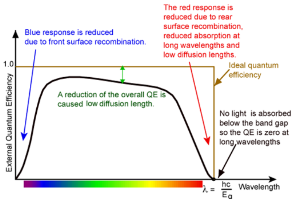
Figure 3.16 EQE curve of a solar cell [107]
