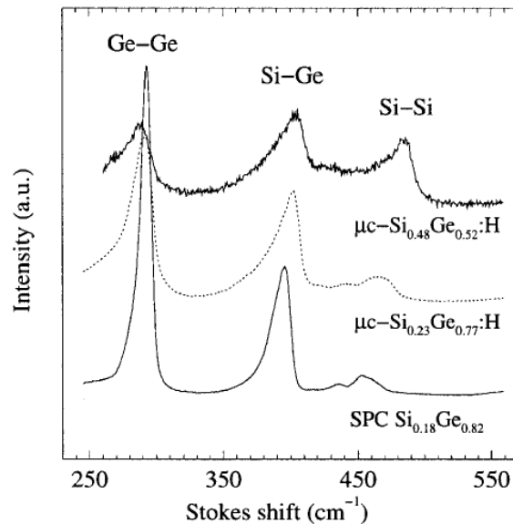
Figure 2.21 Raman spectra of the nc-SiGe:H films with varying Ge content [78]
