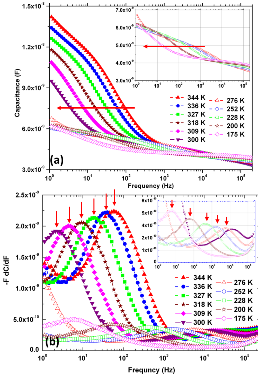
Figure 3. (a) CF at various Temperatures for Perovskite based solar cell. The red arrows indicate the shift in capacitance. (b) Differential capacitance curves. Arrows indicate emission peaks.
