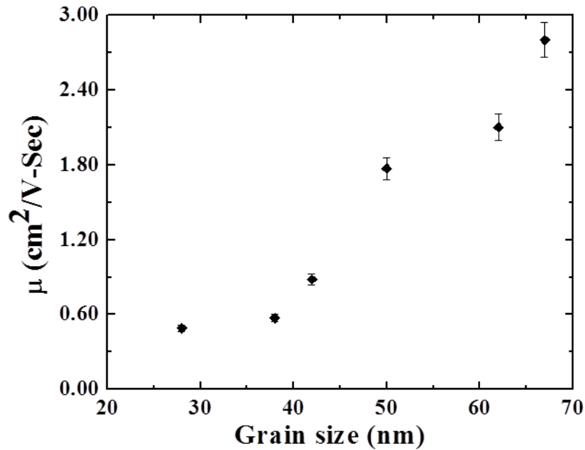
Figure 5. Electron Mobility vs. <220> Grain size
