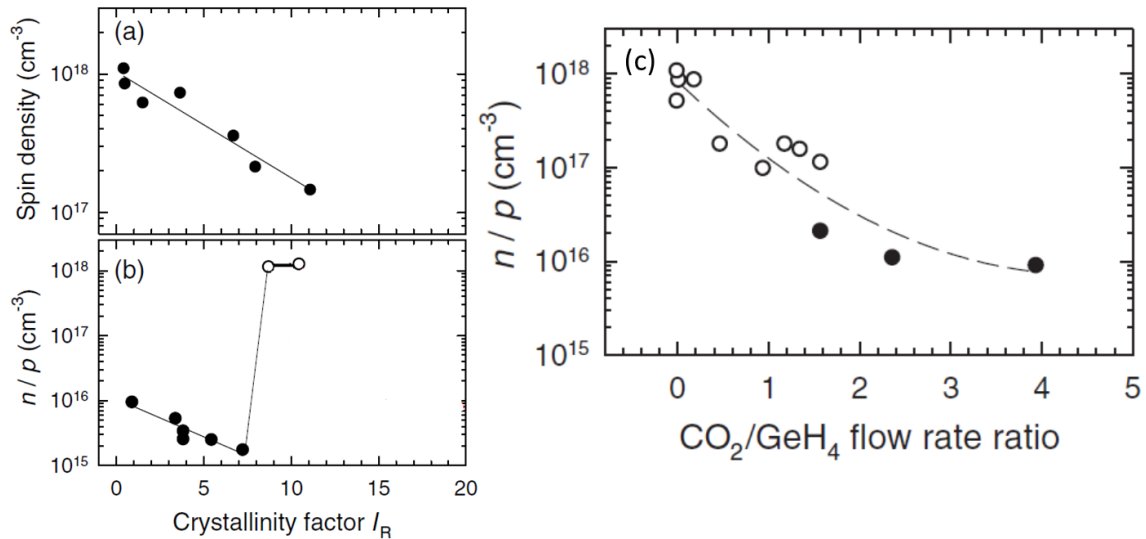
Figure 2.27 (a) ESR spin density, (b) carrier concentration as a function of I R in nc-Ge:H film and (c) carrier concentration as a function of CO 2 gas flow during deposition. n (closed symbols)/p (open symbols) [85]
