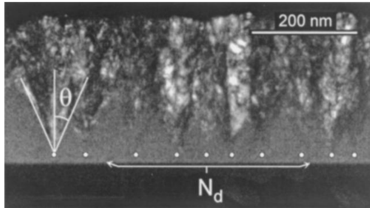
Figure 1.4 TEM image of growth of nc-Si:H showing conical growth [13]
