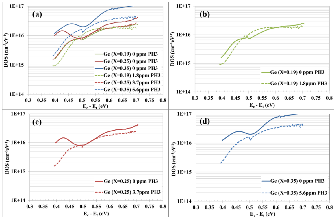
Figure 4.32 (a) Defect density profile in nc-SiGe:H devices with and without PH_3 compensation for varying Ge content, (b) for X_{Ge} = 0.19 , (c) for X_{Ge} = 0.25 , (d) X_{Ge} = 0.35
