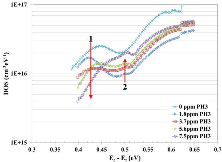
Figure 4.31 Calculated defect density vs. energy below the conduction band for nc-SiGe:H solar cells ( X_{Ge} \sim 0.35 ) for varying PH_3 flow rates
