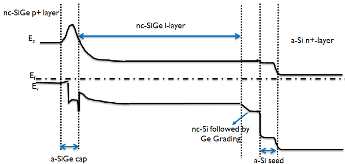
Figure 4.11 Band diagram of nc-SiGe:H device.
