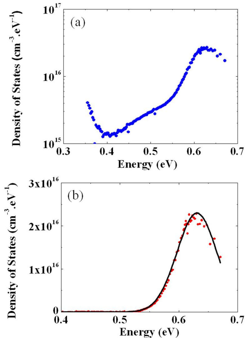
Figure 5 (a) Calculated defect density from CF data at 300K for a Perovskite solar cell and (b) Fitted Gaussian curve for the same data on a linear plot
